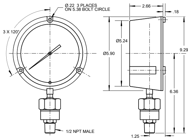
4.5" Turret with Male Mini-Seal
