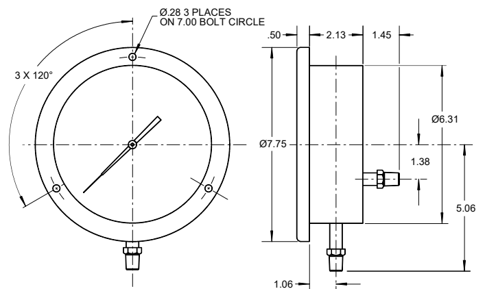
6" Front Flange
